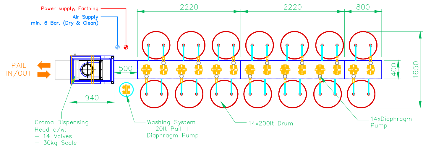
SYSTEM LAYOUT PLAN VIEW
