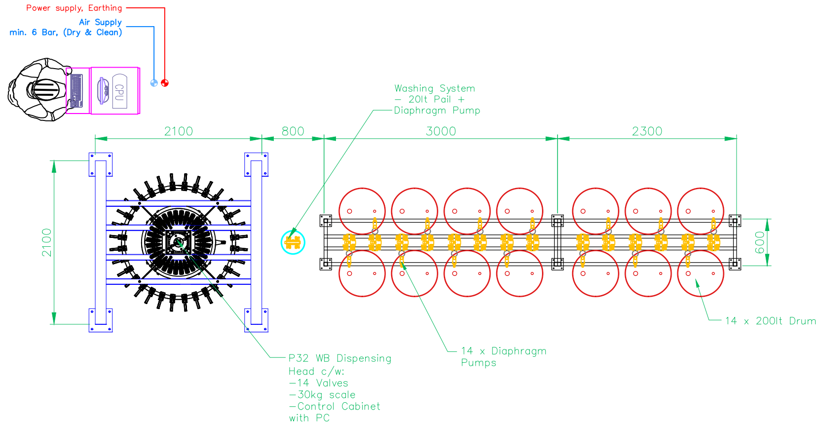
SYSTEM LAYOUT PLAN VIEW
