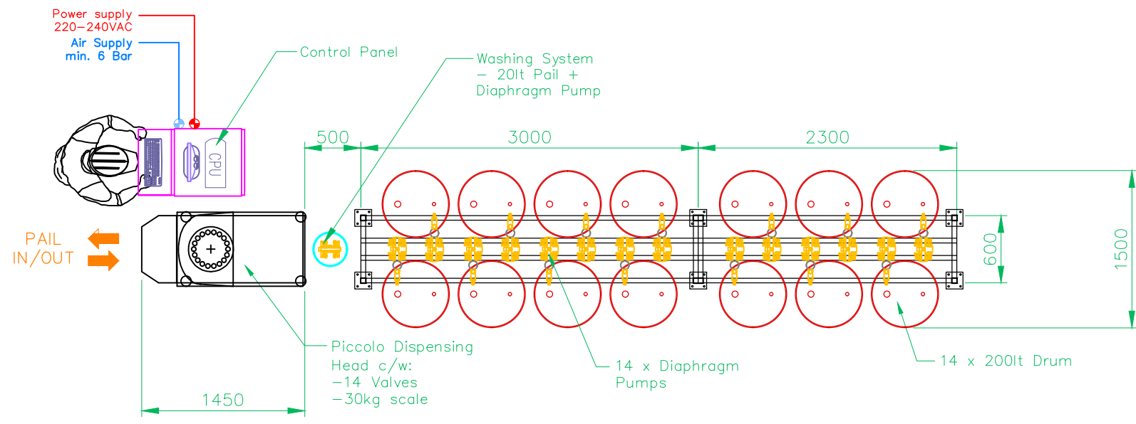
SYSTEM LAYOUT PLAN VIEW
