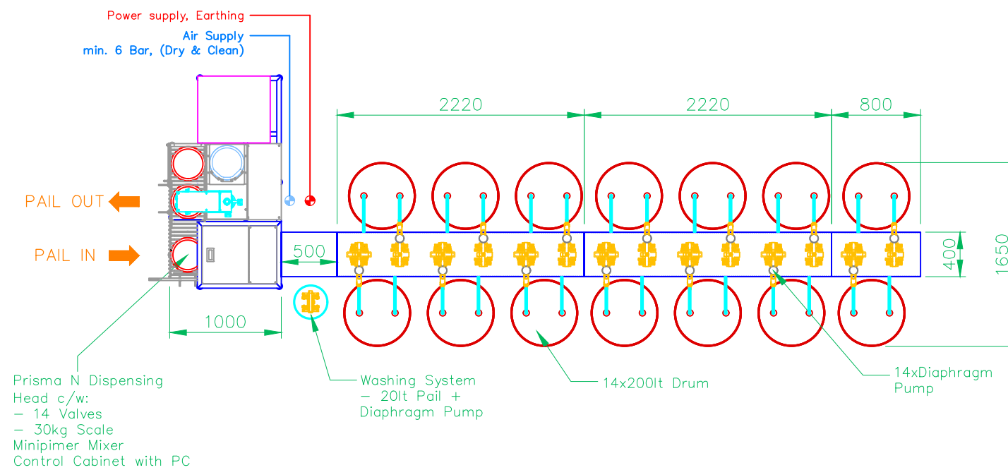
SYSTEM LAYOUT PLAN VIEW
